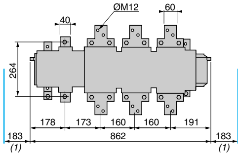
LC1 F78041
