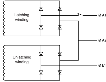
Scheme of internal circuit
