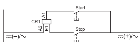
Pushbutton control
