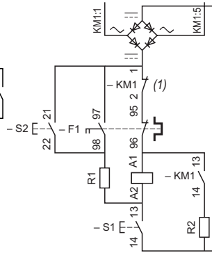
Contactors CR1 B
