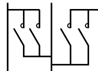
'W' connection
