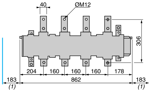
LC1 F78041
